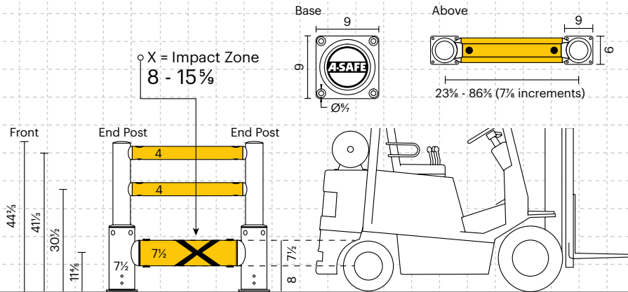
Dimensions (inches)
