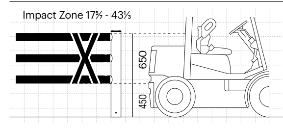
iFlex Cold Storage Pedestrian Guardrail 3 Rail
