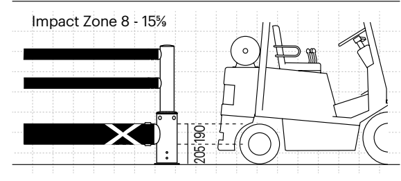
iFlex Cold Storage Single Traffic Guardrail+
