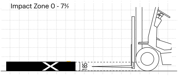
ForkGuard Cold Storage Kerb Guardrail
