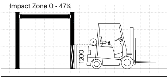
iFlex Cold Storage Height Restrictor
