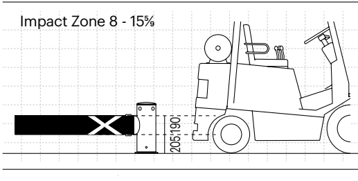
iFlex Cold Storage Single Traffic Guardrail
